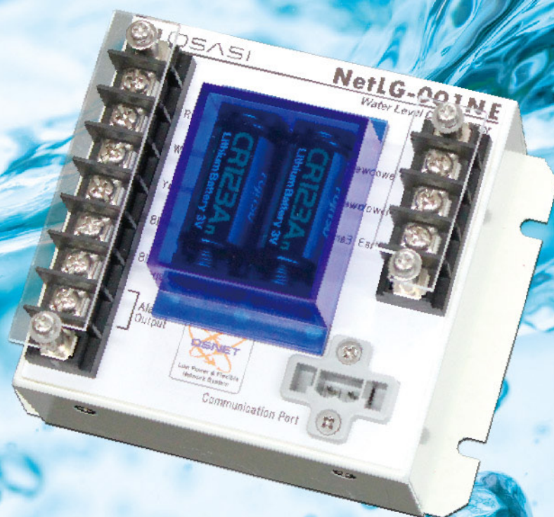
Used with one pressure-type water level sensor (OSASI Technos)
